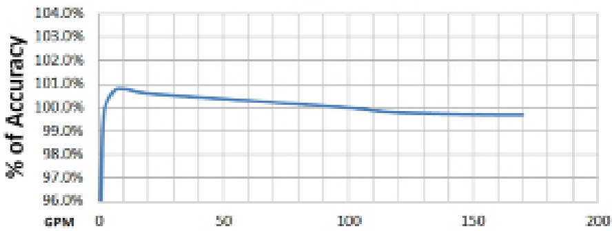
Q&B Meter Performance & Accuracy Curves Positive Displacement Meters 2"
